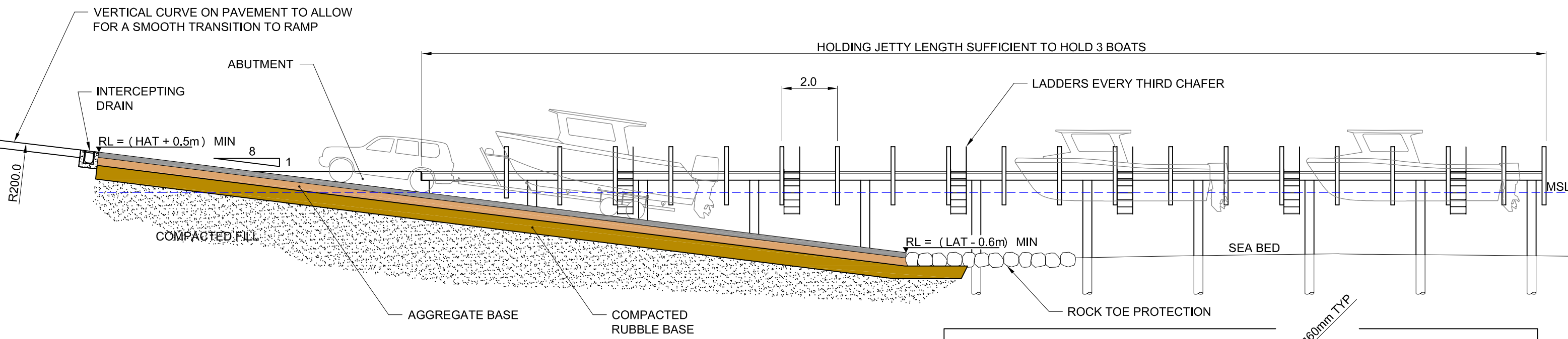
TYPICAL LONGITUDINAL RAMP SECTION
