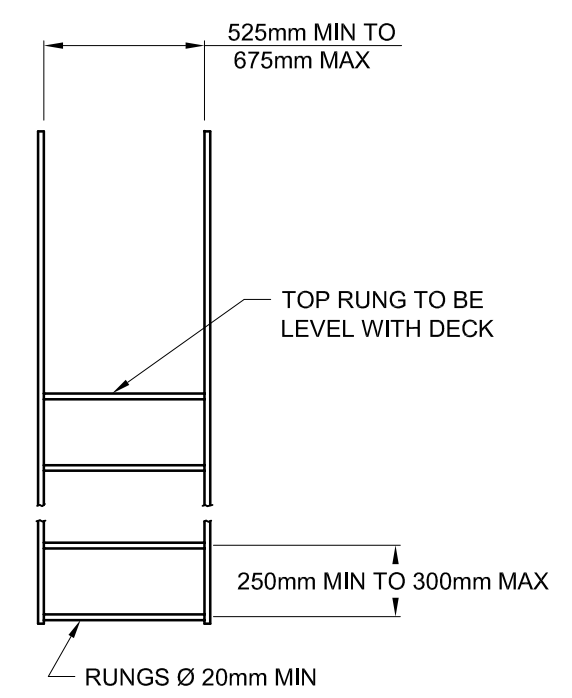
LADDER DETAIL
