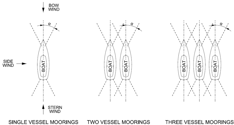
Figure 1: Schematic Vessel Mooring Arrangements for the purpose of determining line loads
