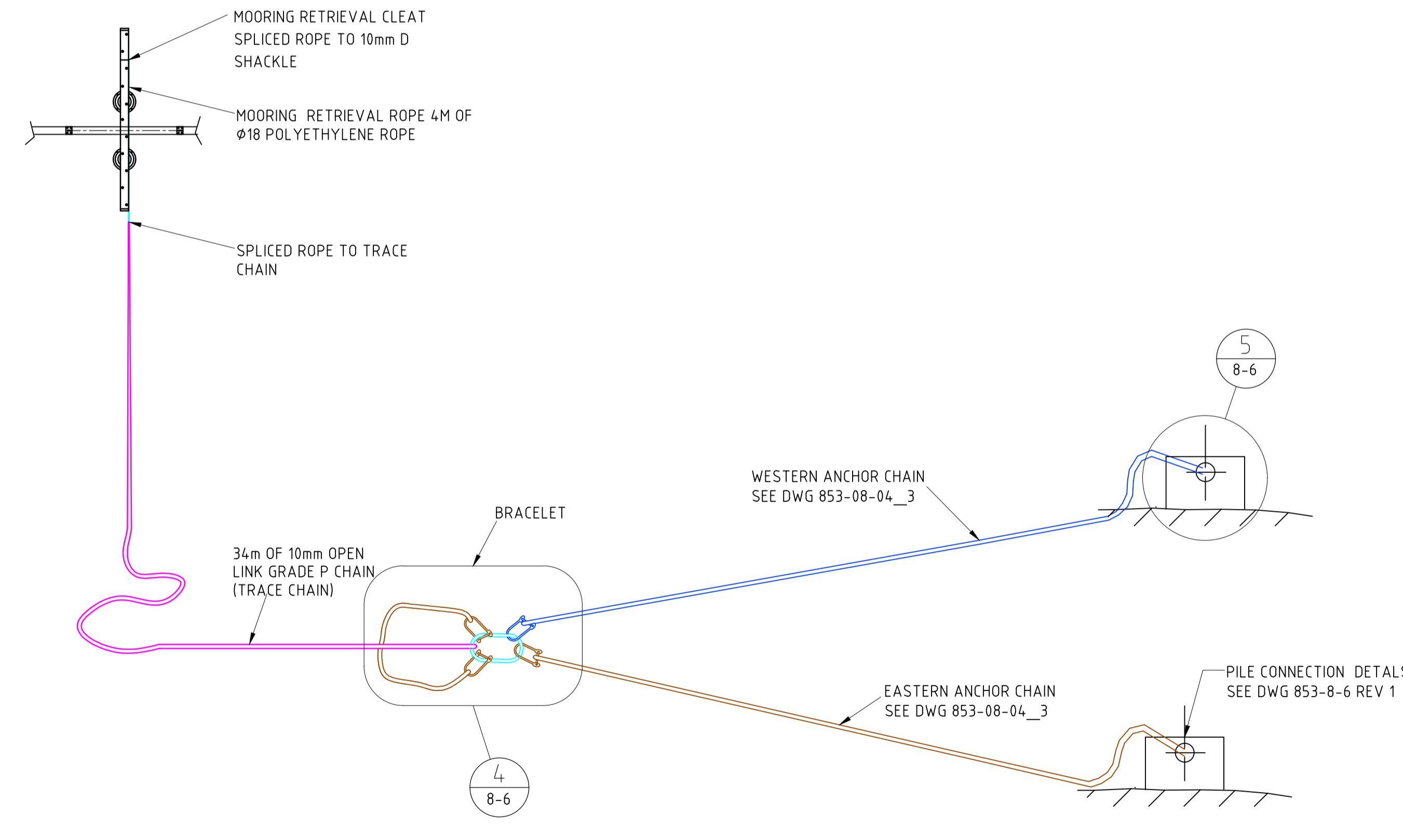
25m MOORING ANCHOR CHAIN ASSEMBLY AND POLYETHYLENE ROPE AND TRACE CHAIN
