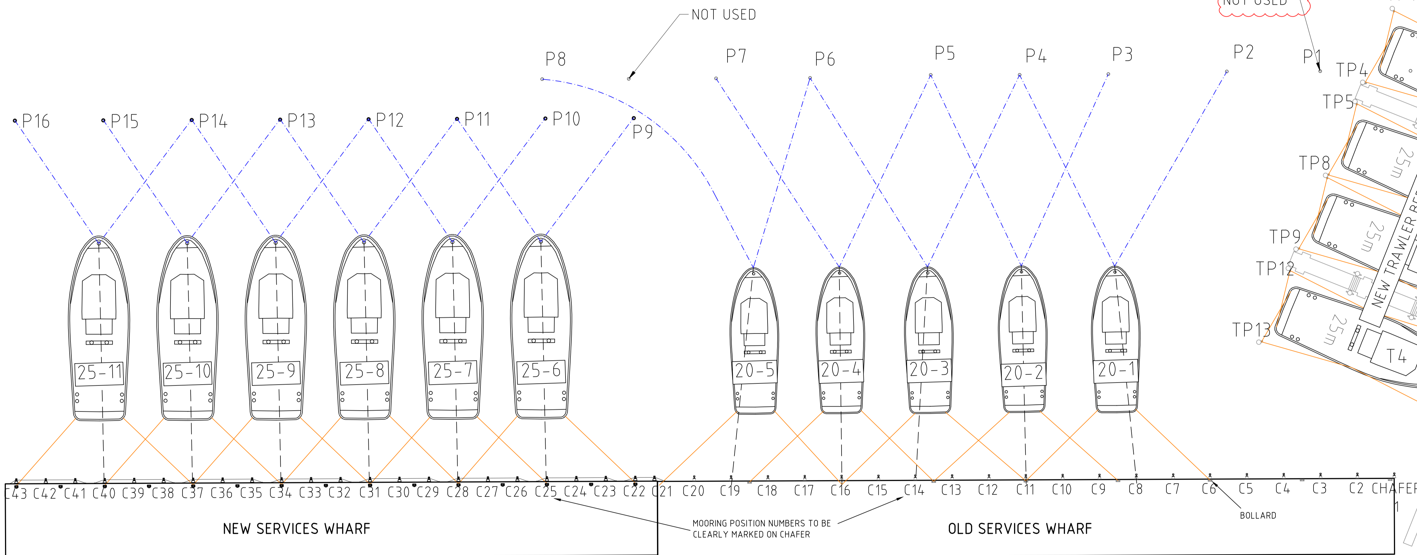
PLAN VIEW SCALE 1:300 (SEE DWG 853-8-1 FOR PERSPECTIVE VIEW)
