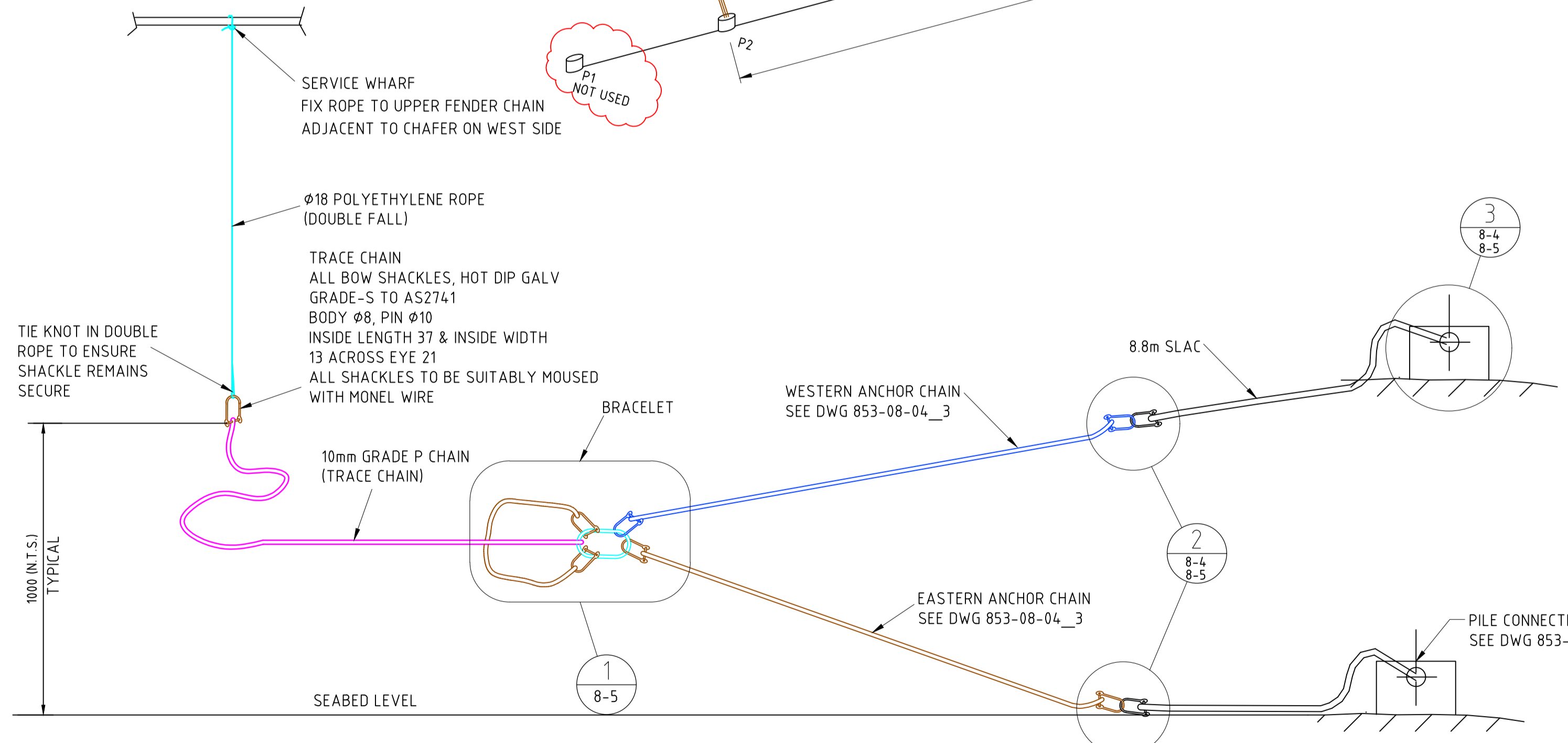
20m MOORING ANCHOR CHAIN ASSEMBLY AND POLYETHYLENE ROPE AND TRACE CHAIN
