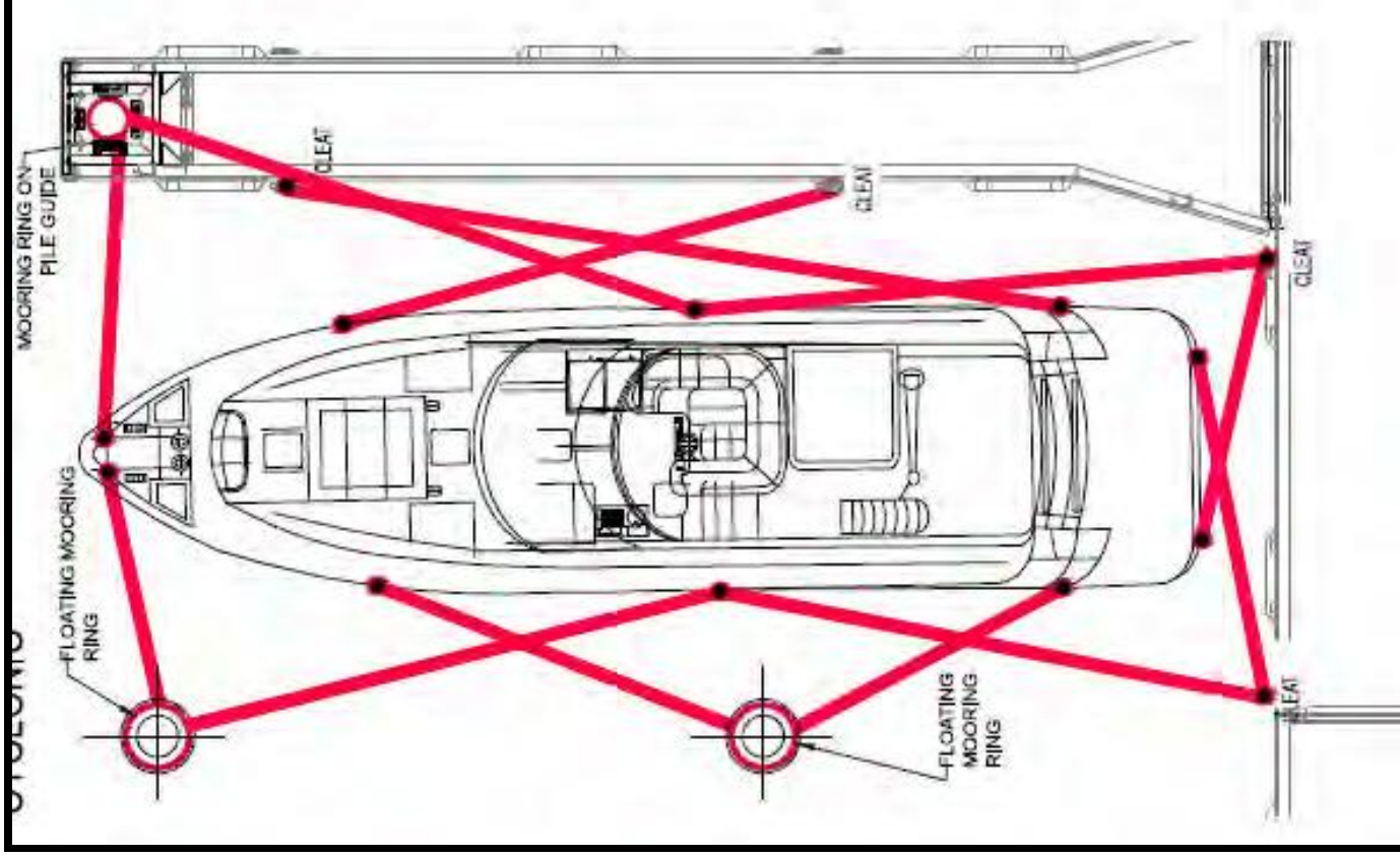
Figure 5: Minimum Mooring Guideline for 25 Metre Jetty B Pens in Cyclonic Conditions
