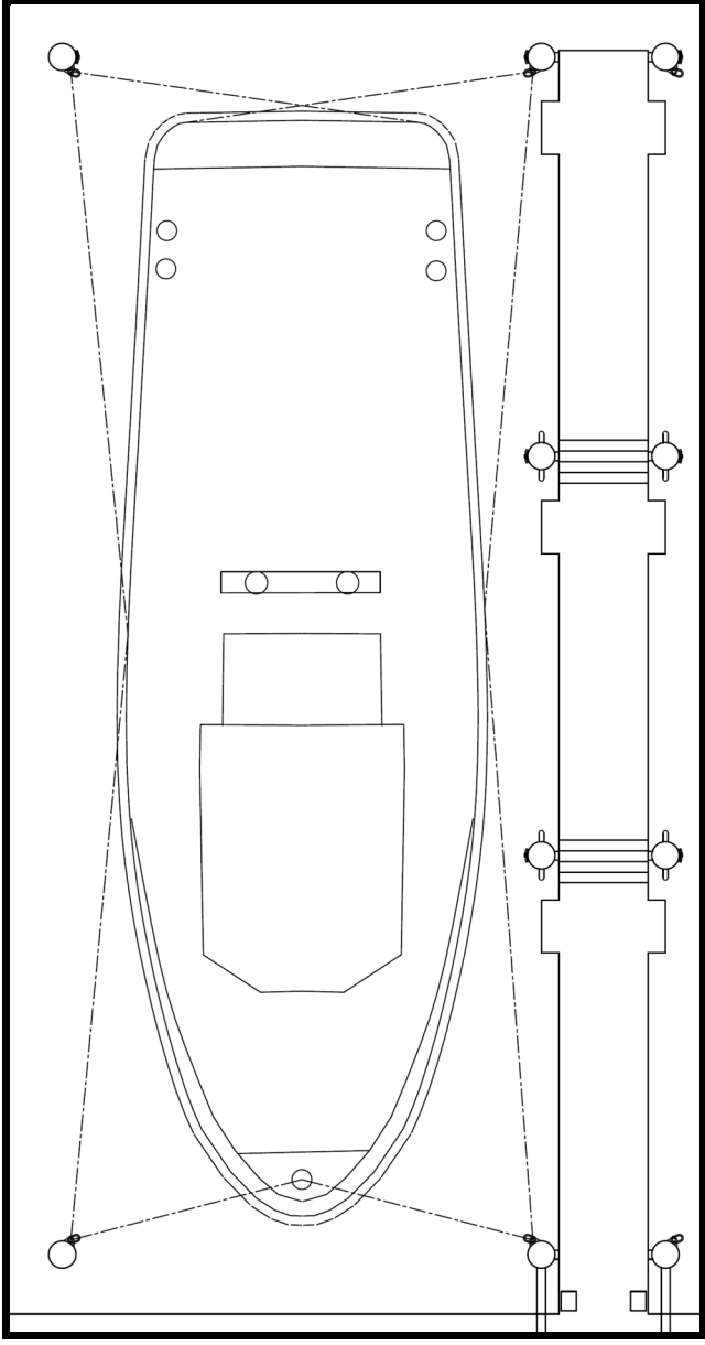
Figure 7: Minimum recommended Mooring Guideline for Charter Boat Pens in Cyclonic Conditions
