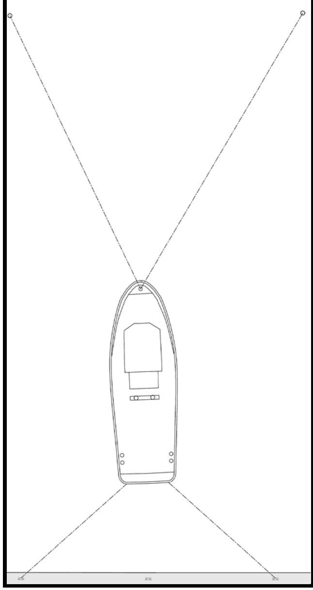
Figure 9: Minimum recommended Mooring Guideline for a Boat to the Service Wharf in Cyclonic Condition
