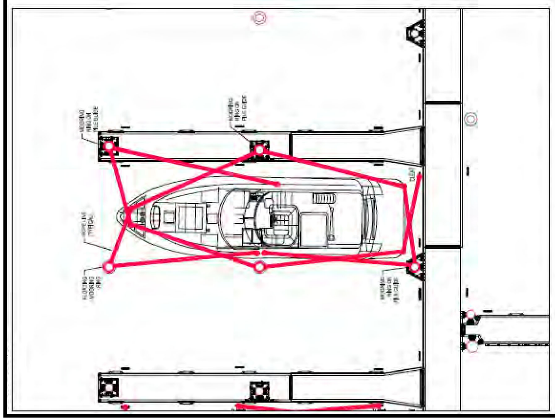
Figure 4: Minimum Mooring Guideline 20 Metre Jetty B Pens in Cyclonic Conditions
