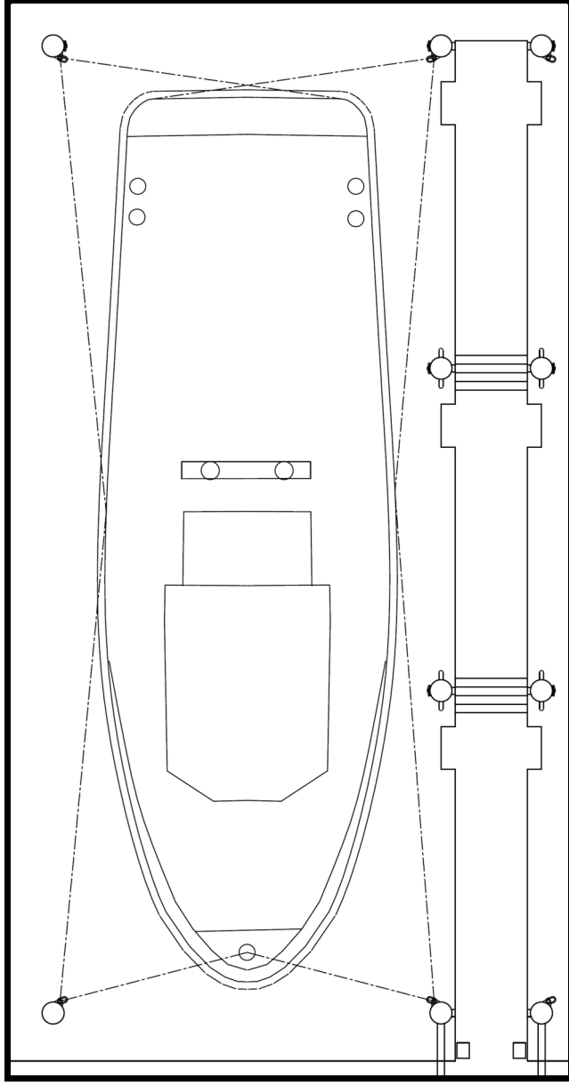
Figure 8: Minimum recommended Mooring Guideline for Trawler Pens in Cyclonic Conditions
