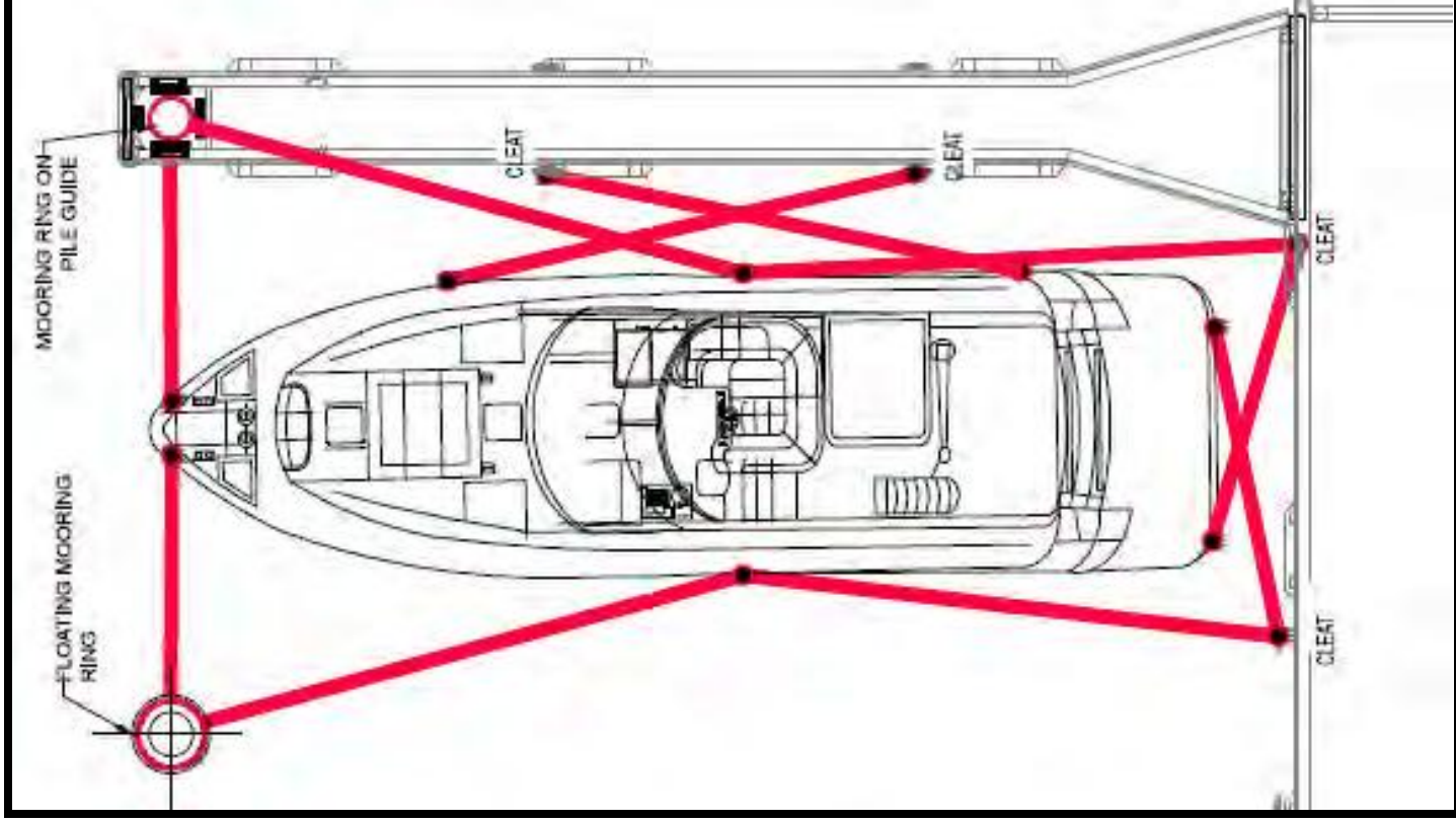
Figure 6: Minimum Mooring Guideline for 12 to 15 Metre Jetty B Pens in Cyclonic Conditions
