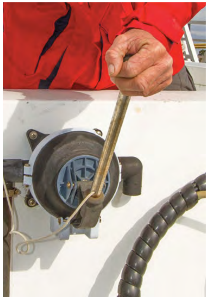
A bilge pump can be manually, electrically or mechanically operated
