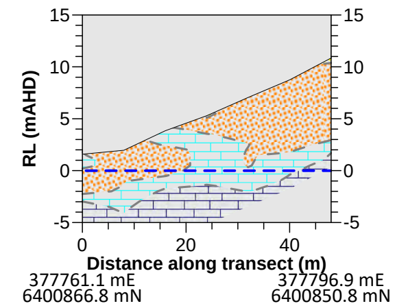
TRANSECT 7 - INTERPRETED GEOLOGICAL SECTION
