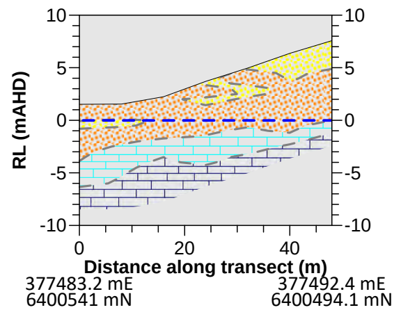
TRANSECT 5 - INTERPRETED GEOLOGICAL SECTION
