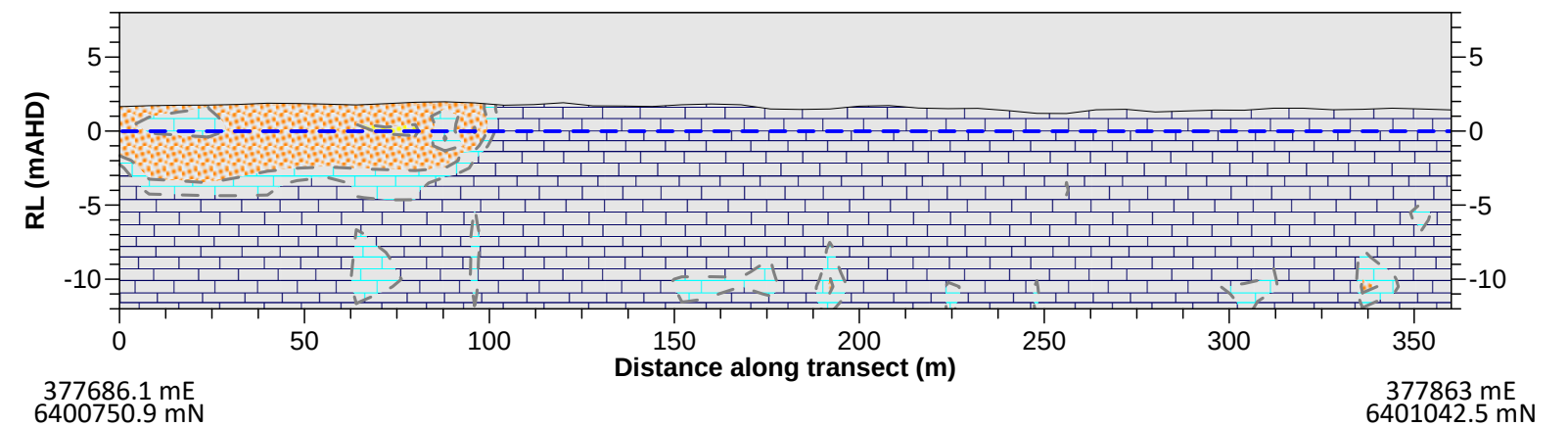
TRANSECT 2 (0-360m) - INTERPRETED GEOLOGICAL SECTION
