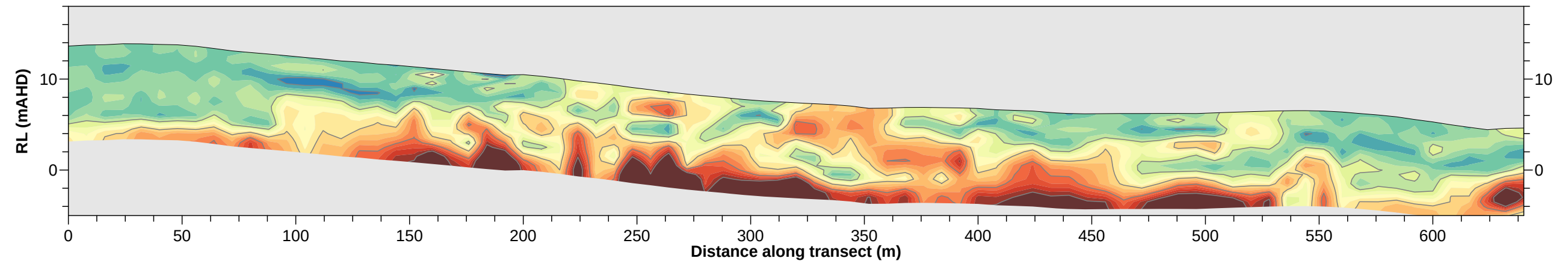
TRANSECT 4 - SEISMIC SHEAR WAVE VELOCITY MODEL
