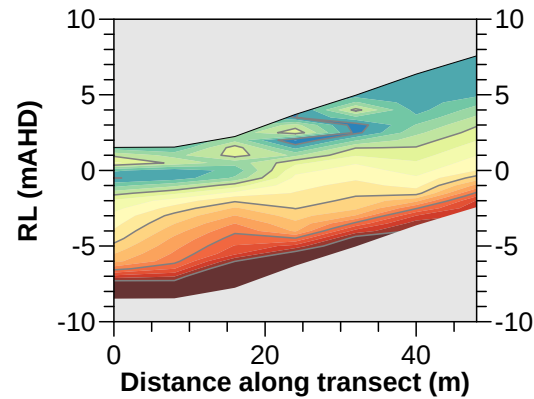
TRANSECT 5 - SEISMIC SHEAR WAVE VELOCITY MODEL
