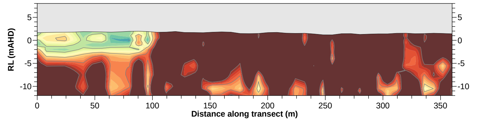
TRANSECT 2 (0-360m) - SEISMIC SHEAR WAVE VELOCITY MODEL
