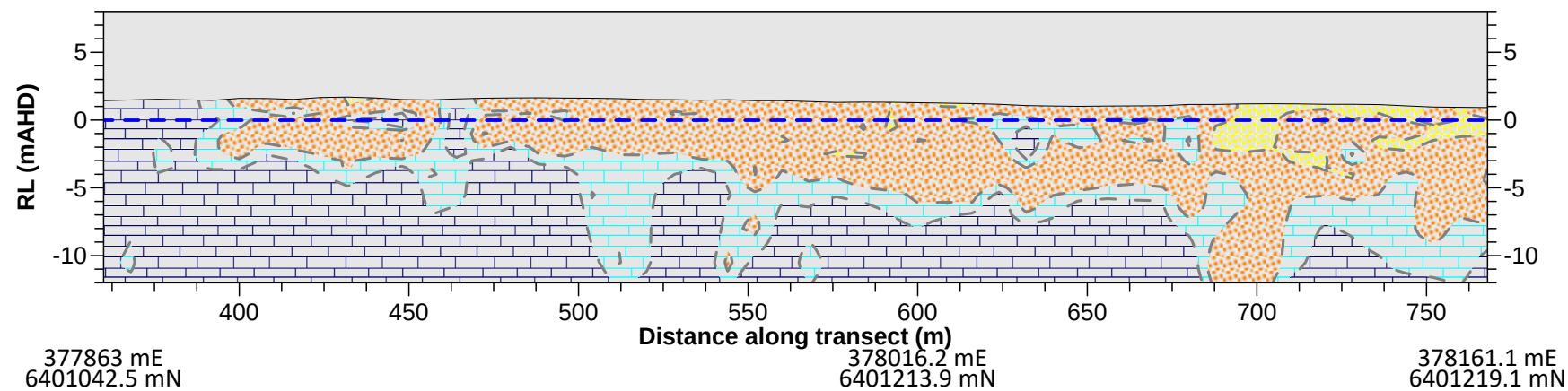
TRANSECT 2 (360-768m) - INTERPRETED GEOLOGICAL SECTION
