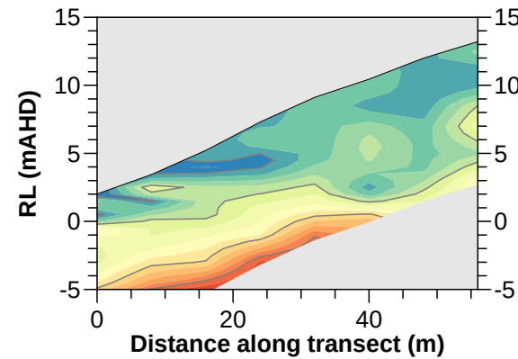
TRANSECT 6 - SEISMIC SHEAR WAVE VELOCITY MODEL
