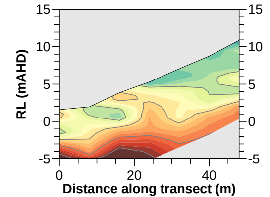
TRANSECT 7 - SEISMIC SHEAR WAVE VELOCITY MODEL
