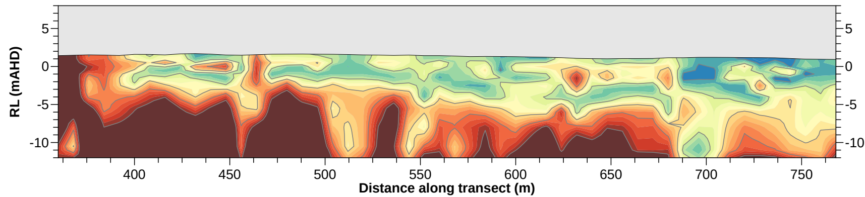
TRANSECT 2 (360-768m) - SEISMIC SHEAR WAVE VELOCITY MODEL
