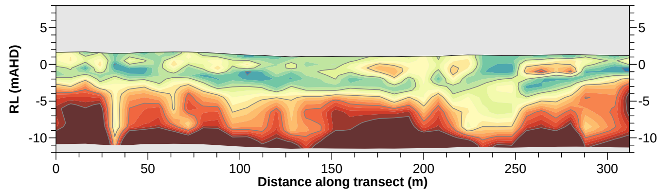
TRANSECT 1 - SEISMIC SHEAR WAVE VELOCITY MODEL
