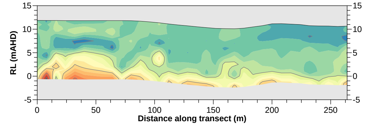
TRANSECT 3 - SEISMIC SHEAR WAVE VELOCITY MODEL
