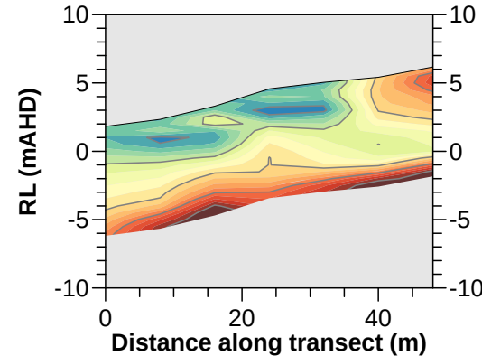
TRANSECT 8 - SEISMIC SHEAR WAVE VELOCITY MODEL
