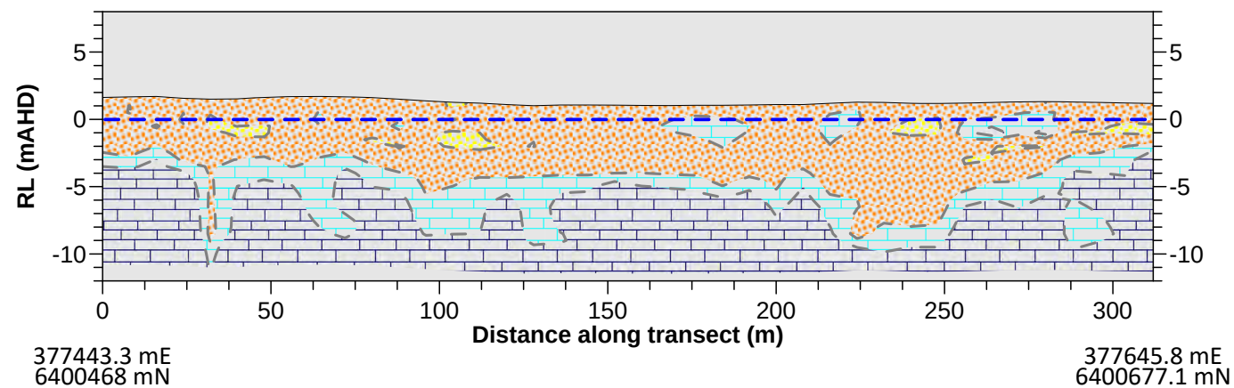
TRANSECT 1 - INTERPRETED GEOLOGICAL SECTION
