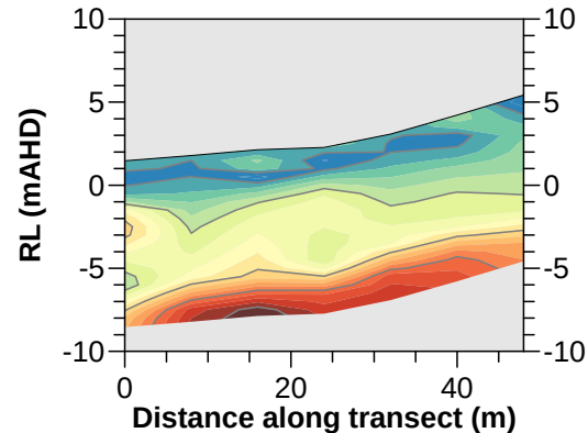
TRANSECT 9 - SEISMIC SHEAR WAVE VELOCITY MODEL
