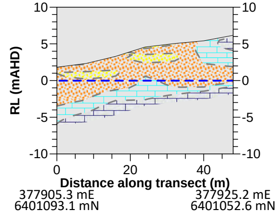
TRANSECT 8 - INTERPRETED GEOLOGICAL SECTION
