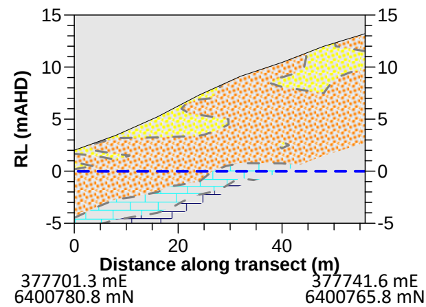
TRANSECT 6 - INTERPRETED GEOLOGICAL SECTION
