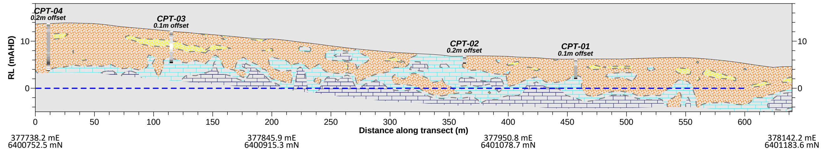
TRANSECT 4 - INTERPRETED GEOLOGICAL SECTION
